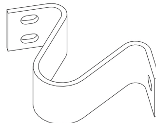
AXONOMETRY VIEW
